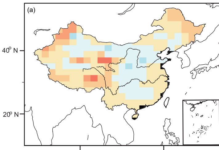
JJA mean temperature
