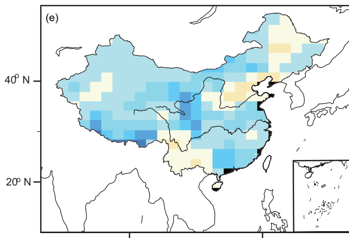
DJF mean precipitation
