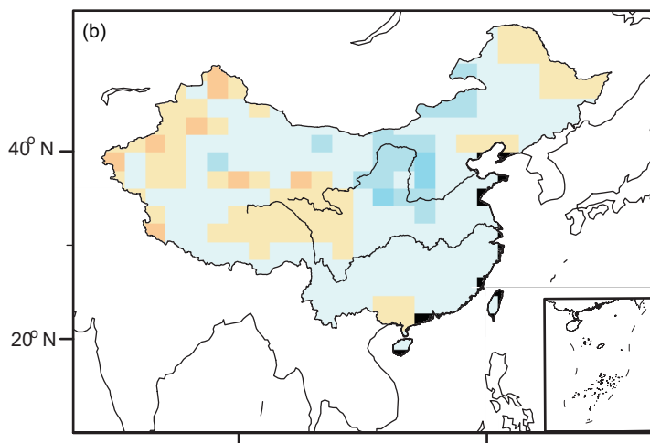
DJF mean temperature
