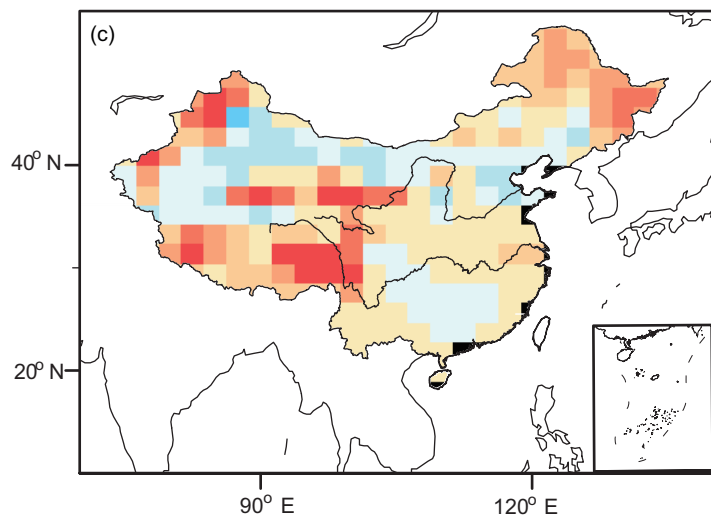
DJF mean temperature
