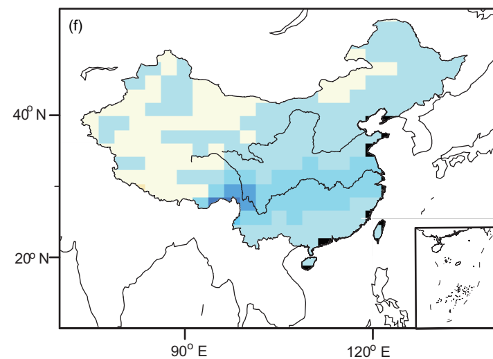
DJF mean precipitation
