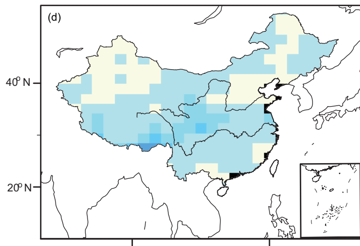
JJA mean precipitation
