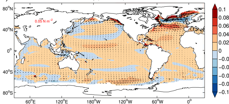
b) ANN Surface wind stress anomaly (MIS3 – PI)
