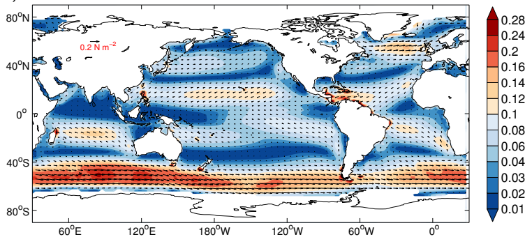
a) ANN Surface wind stress (PI control)
