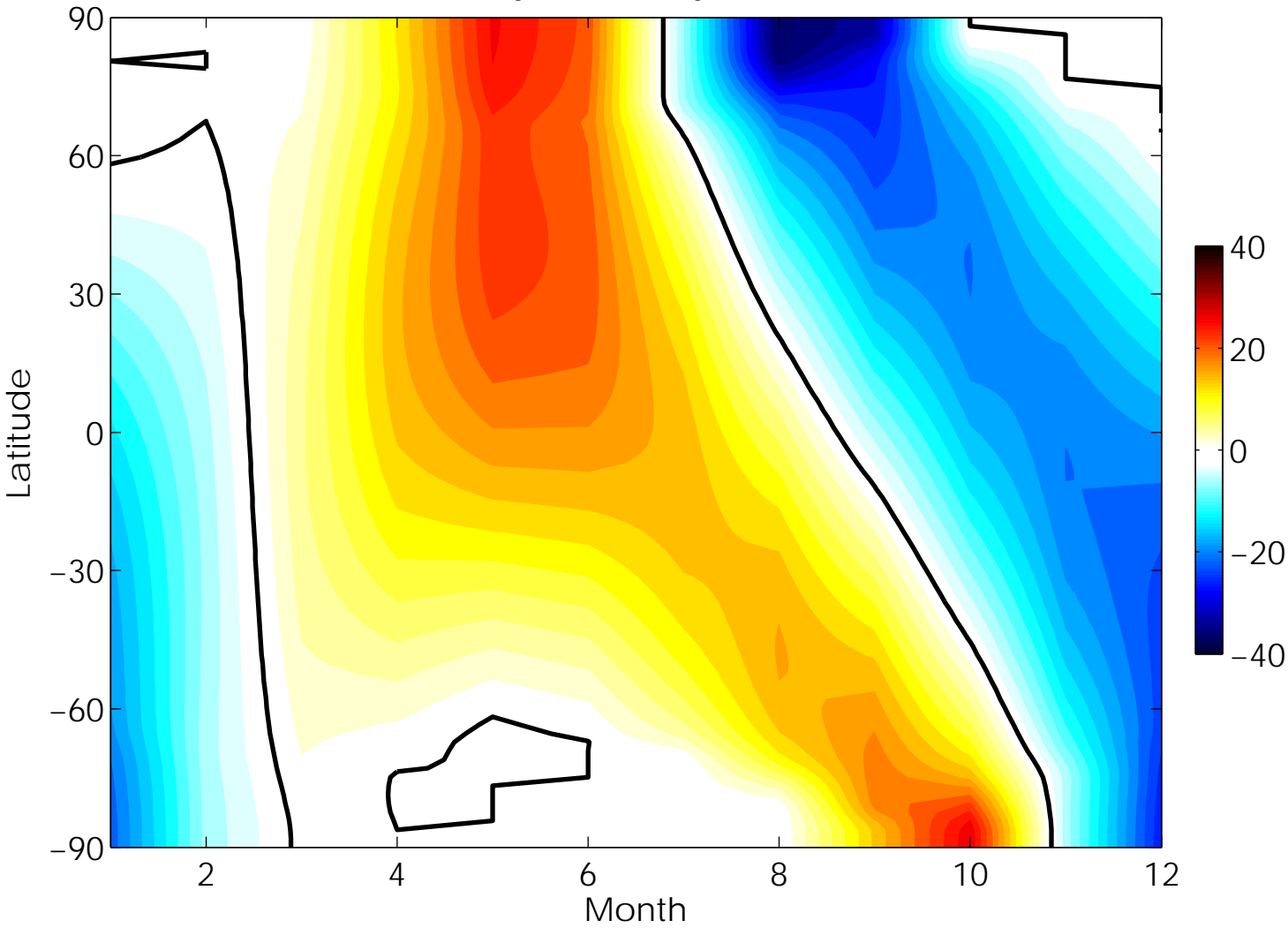
Insolation anomaly: MIS3(38 kyr BP) – PI (W m -2 )
