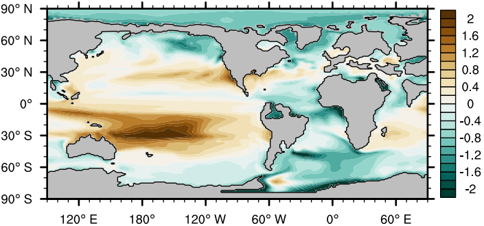
(c) Evap - precip 1600 — 800 ppm ( 10^{-5} \text{ kg m}^{-2} \text{ s}^{-1} )
