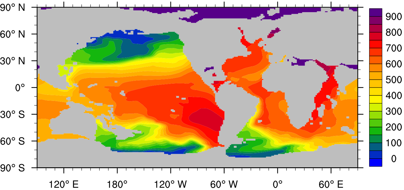
(b) Mixed layer depth (m)
