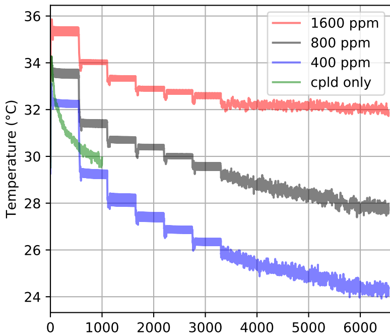
(c) Temp 4000 m
