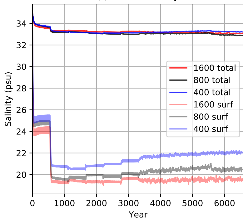
(f) Arctic salinity
