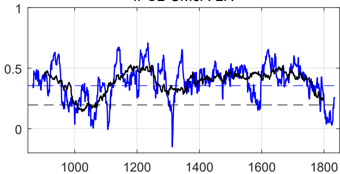
IPSL-CM5A-LR
