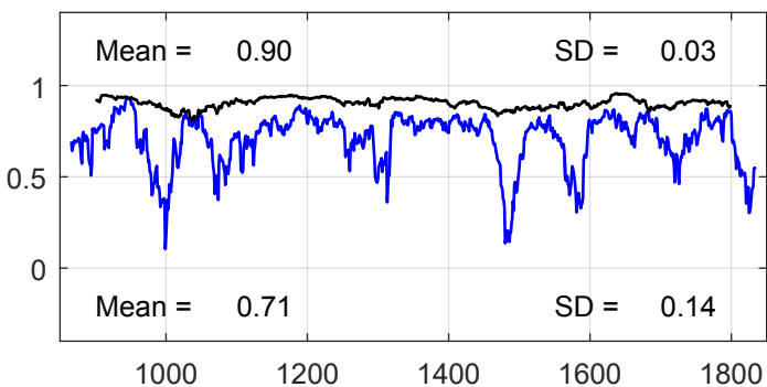
IPSL-CM5A-LR
