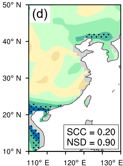
IPSL-CM5A-LR
