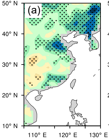
FGOALS-s2
