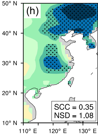
IPSL-CM5A-LR
