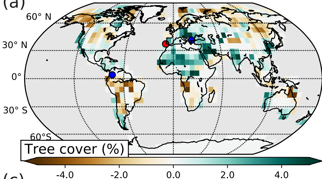
OVC: fixed ice sheets
