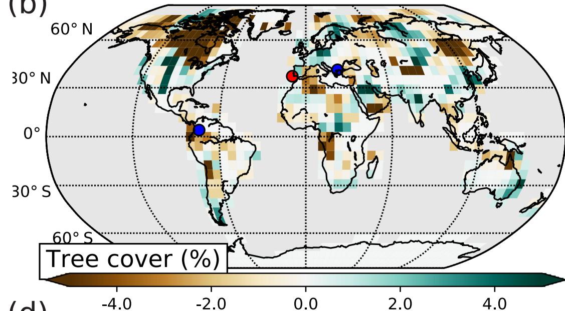
OVIC: different ice sheets
