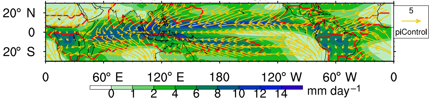
(b) ND mean precp (piControl climatology)
