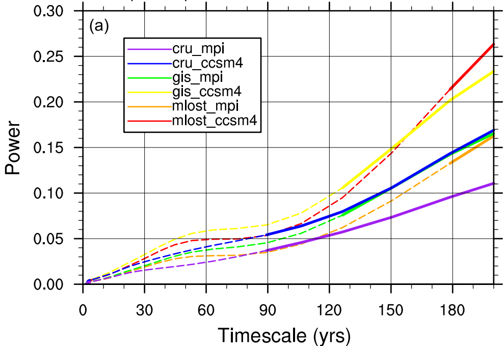
Global power spectrum
