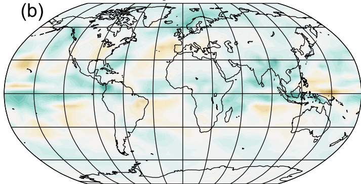
In LMR, yrs 1850 to 2000
