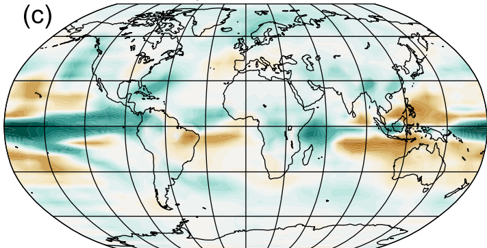
In LMR, yrs 1200 to 1850
