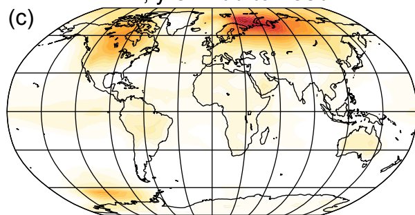
Prior, ccsm4, no filt
