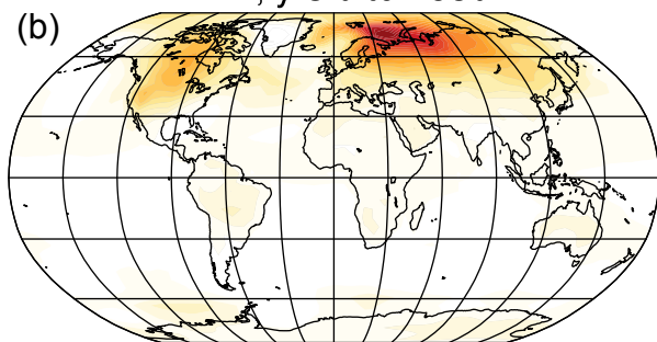
LMR, yrs 1850 to 2000
