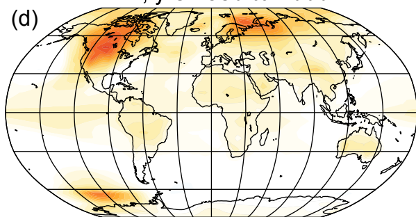
LMR, yrs 0 to 1850, no filt
