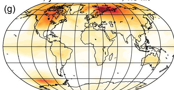
LMR, yrs 1200 to 1850, no filt
