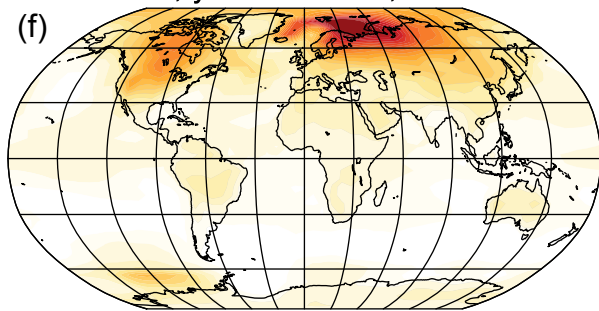
LMR, yrs 1850 to 2000, no filt
