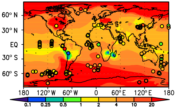
(b) \text{LGM}_{\text{glac.}a}/\text{PI}_a
