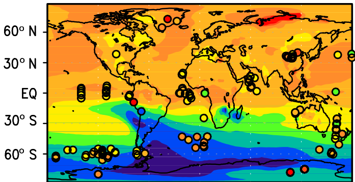
(a) \text{LGM}_a/\text{PI}_a
