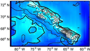
(a) Cloud radiative forcing (bin It1)
