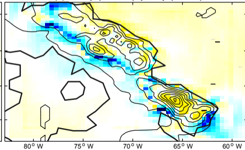
(c) Precip (bin It10)–precip (bin It1)
