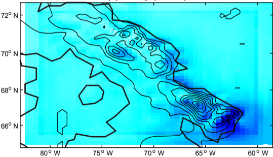
(a) Precip (bin It1)
