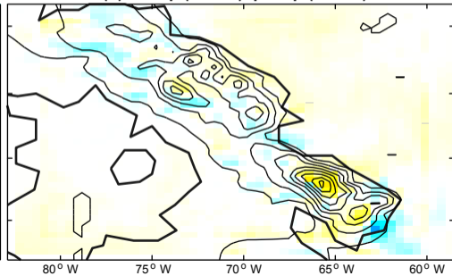
(b) Precip (bin It2)–precip (bin It1)
