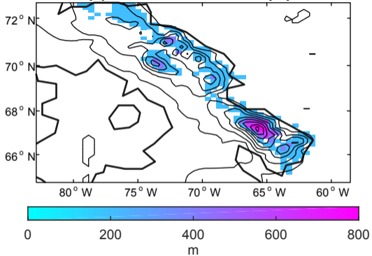
(a) Initial ice thickness (m)
