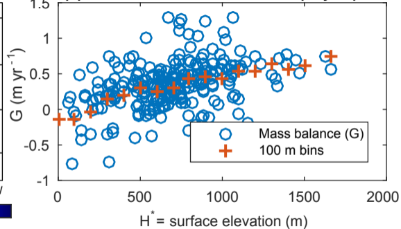
(c) It. 1 WRF annual mass bal. (m yr -1 )
