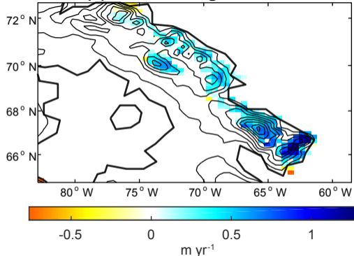
(b) Mass bal. avg. = 0.35087
