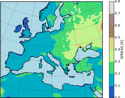
(c) Ensemble spread for summer
