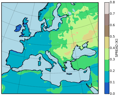
(c) Ensemble spread for summer
