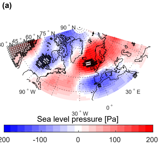
Solar 11-year cycle min-max
