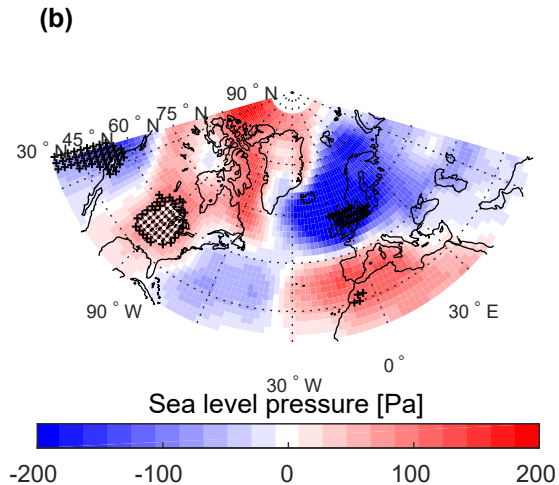
5-year time lag
