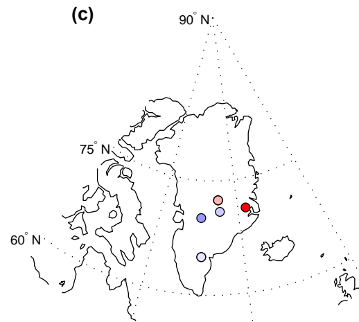
Ice core PC3
