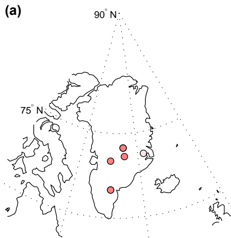
Ice core PC1
