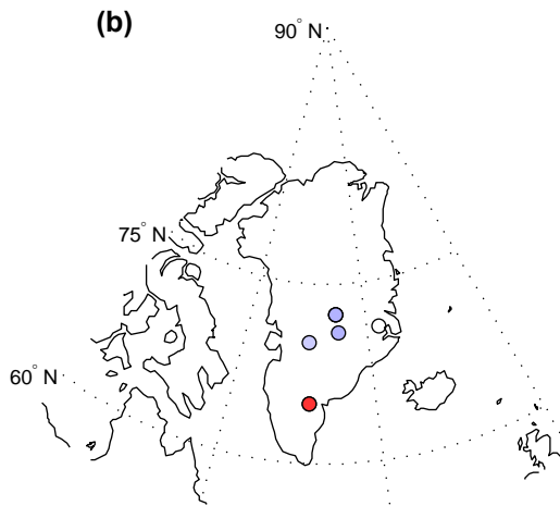
Ice core PC2
