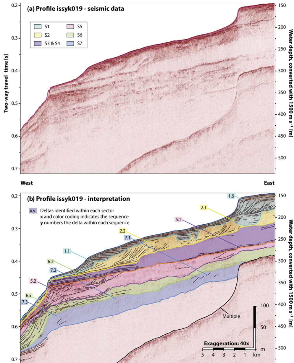
Figure 6. Seismic profile issyk019. Upper panel: seismic data. Lower panel: line drawing and interpretation of all sequences identified in the profile. All delta lobes identified in issyk019 are indicated. One delta lobe was spotted in S6 but could not be clearly identified because it is too eroded. This delta lobe is marked as 6.x in the figure and was not considered for the reconstruction of the lake-level curve. See figure 1 for location of profile issyk019.
