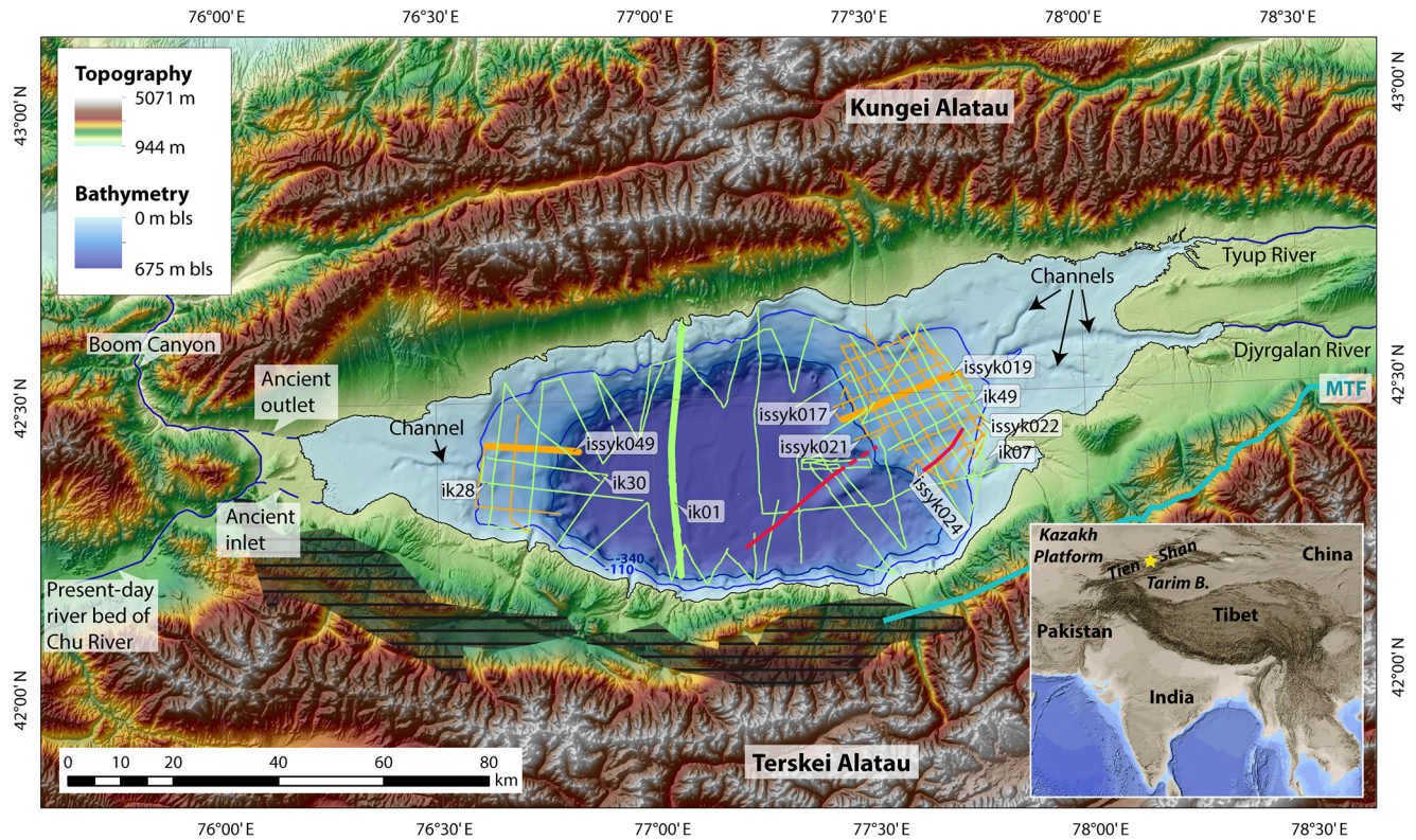
Figure 1. Geographical setting of Lake Issyk-Kul. Track lines of all profiles used in this study are shown in green (data from 1997) and orange (2001). Profiles shown in Figs. 3–6 and 8 are shown by bold lines. The axes of two anticline structures visible in the seismic profiles in the southeastern part of the lake are marked in red. Grey hatched areas mark the approximate position of the Issyk-Kul broken foreland. Blue line shows the approximate location of the main Terskey Fault (MTF; after Macaulay et al., 2014). Digital terrain model for the lake and surroundings from Delvaux et al. (2001). Bathymetry is given in meters below lake surface (m bls). Inset shows the location of our study site marked by a yellow star (map generated using the ETOPO1 dataset, Amante and Eakins (2009), projection: WGS84 UTM Zone 43N).
