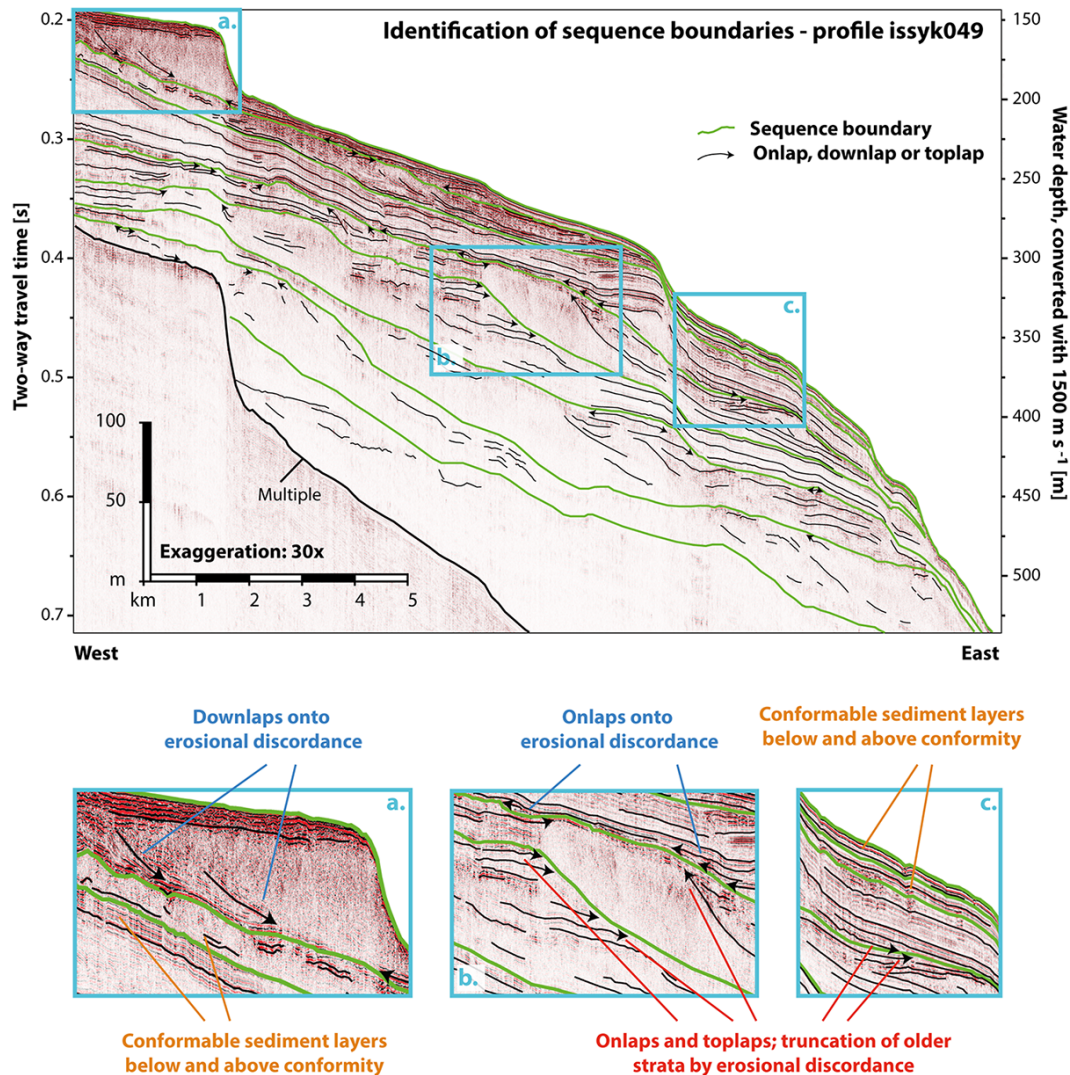
Figure 3. Identification of sequence boundaries of Lake Issyk-Kul sediments. Sequence boundaries could best be determined in places where underlying strata were truncated by erosion, and strata hence form onlaps or toplaps onto the erosional discordance. Also where overlying strata form downlaps or onlaps onto the stratigraphic boundary these were easily identified. Once identified, stratigraphic boundaries could also be traced as distinct reflections into places where they separate the upper and lower stratigraphic sequence as a conformity.
