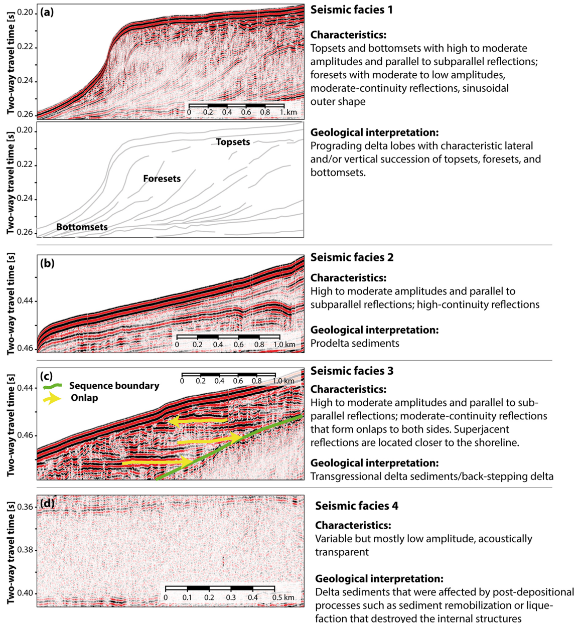
Figure 2. Seismic facies types, SF1–4, of Lake Issyk-Kul sediments. All examples were taken from profile issyk019 (for location of the profile refer to Fig. 1).
