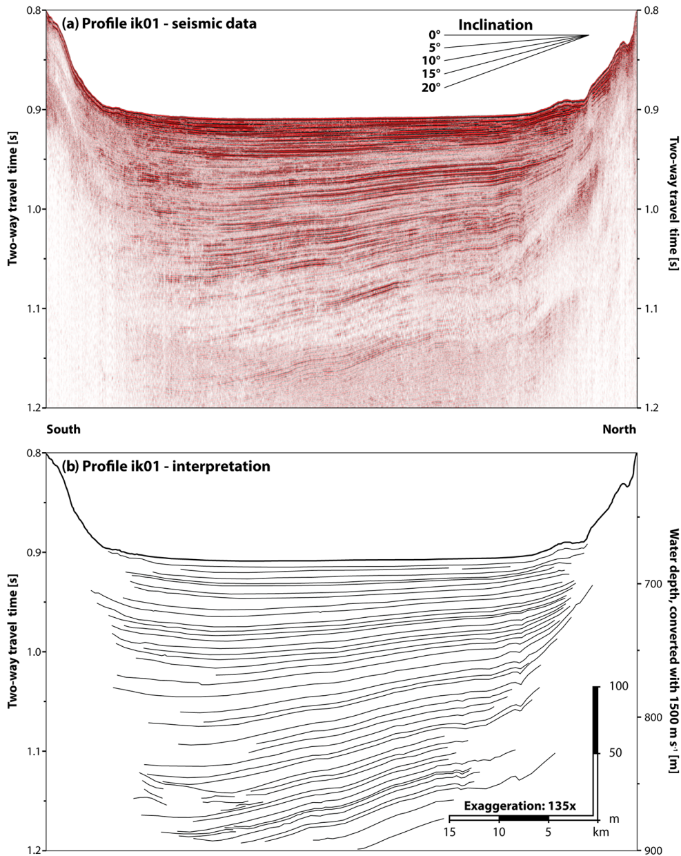
Figure 4. North–south profile ik01. The asymmetric nature of the lake basin is clearly visible with considerably higher subsidence rates towards south.
