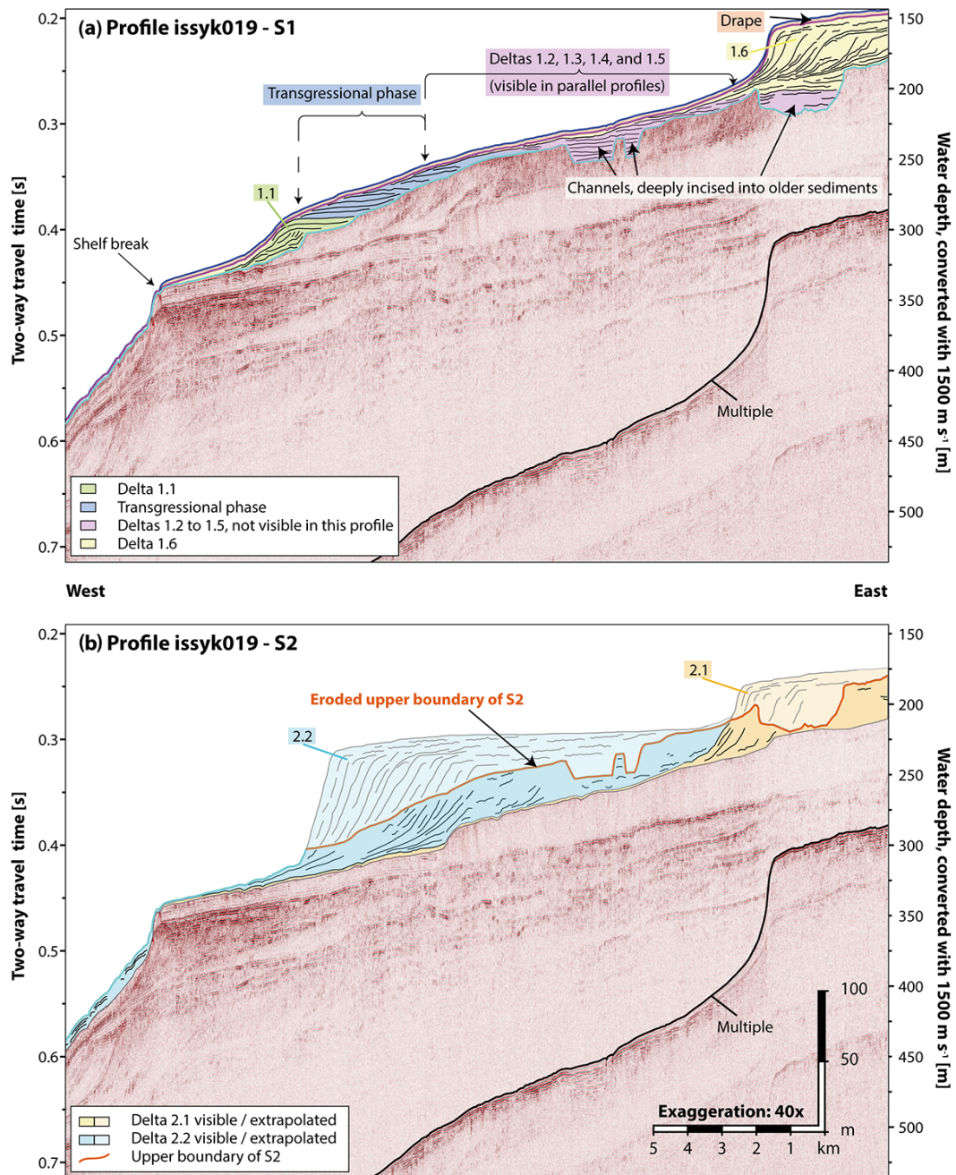
Figure 8. Sequences 1 and 2 on seismic profile issyk019. Upper panel: sequence 1 with distinct deltas 1.1 and 1.6 and the transgressional phase. Deltas 1.2 to 1.5 are only visible in parallel profiles, but their relative location is marked. Note that the lower boundary of Sequence 1 is highly erosive with deeply incised channels. Lower panel: sequence 2. The missing (eroded) parts of deltas 2.1 and 2.2 are tentatively completed in light colors for better visualization. Seismic data overlaying the respective sequences are removed.
