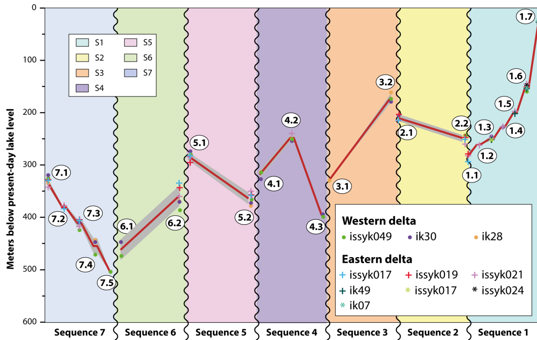
Figure 9. Lake-level curve of Lake Issyk-Kul. Red line: mean value of delta depths. Gray shading: standard deviation of delta depths. Numbers correspond to delta numbers in the text and in Table 1. Boundaries in between the different sequences are at least partially erosive.
