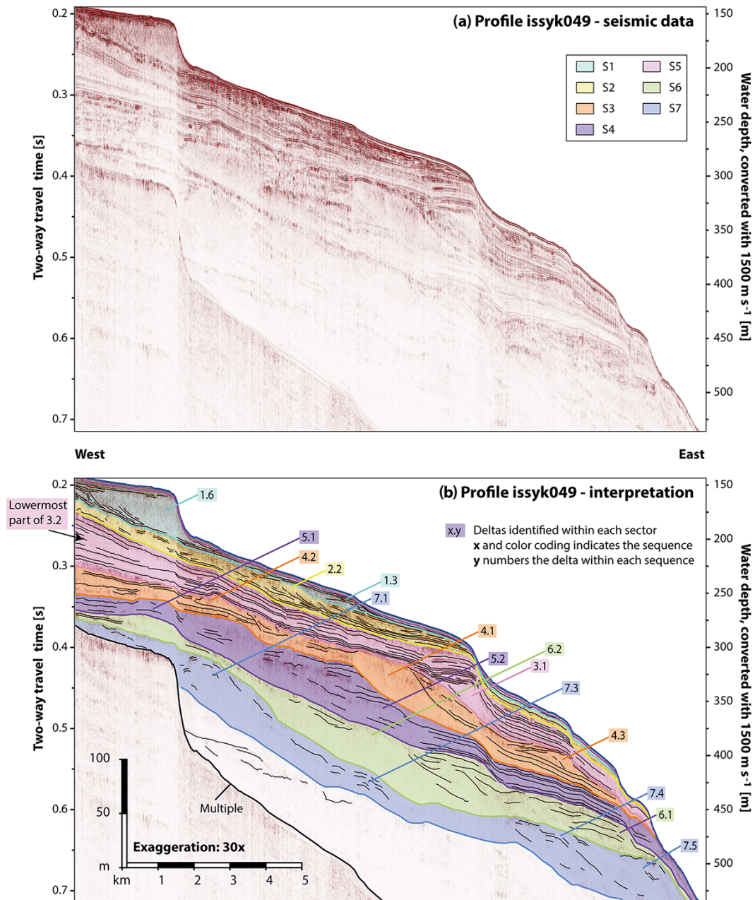
Figure 5. Seismic profile issyk049. Upper panel: seismic data. Lower panel: line drawing and interpretation of all sequences identified in the profile. All delta lobes identified in issyk049 are indicated. See Fig. 1 for location of profile issyk049.
