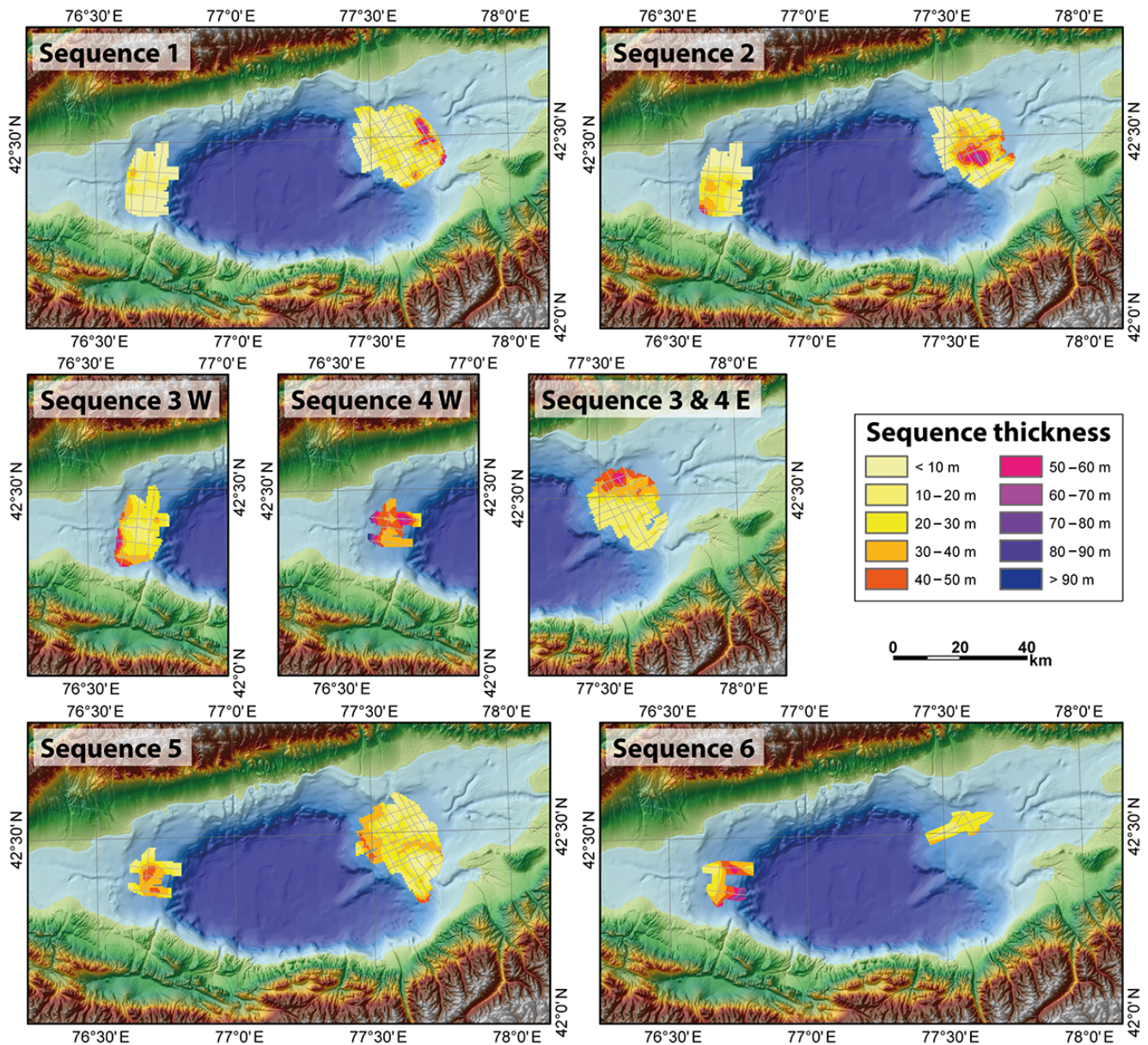
Figure 7. Minimum thickness of sequences in the western and eastern areas. Thickness is converted from two-way travel time using a seismic velocity of 1500 \text{ m s}^{-1} . Thickness color scale is similar for all panels and shown in the figure. Color scales for topography and bathymetry are similar to Fig. 1. Grey lines show where data were available for thickness calculation. Note that sequences 3 and 4 could only be distinguished in the western delta, while a combined thickness for sequences 3 & 4 was calculated for the eastern delta.
