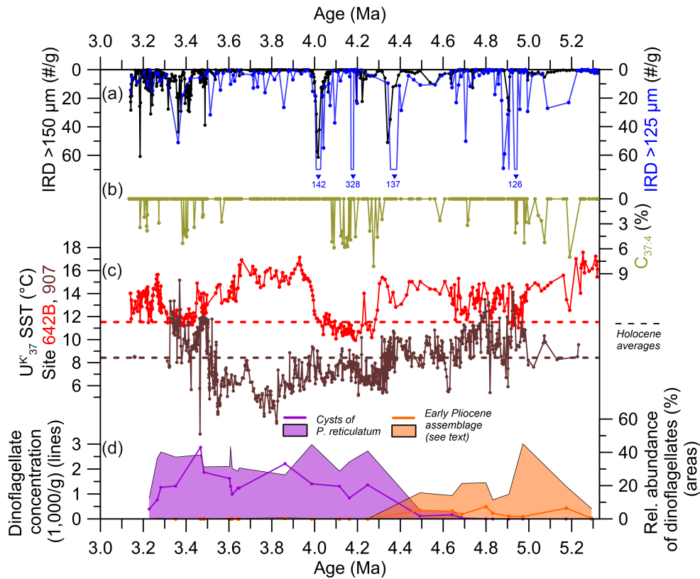
Figure 2. (a) IRD >150 \mu\text{m} (black line, this study) and >125 \mu\text{m} (blue line, Jansen et al., 1990). (b) \%C_{37:4} . (c) U_{37}^{K'} SSTs (Müller et al., 1998 calibration). New data from ODP Hole 642B in red, data from ODP Site 907 in brown (Herbert et al., 2016; age model revised by Clotten et al., unpublished data). Dashed lines indicate Holocene average SSTs for the Norwegian Sea (red: Calvo et al., 2002) at 11.6 ^{\circ}\text{C} , and for the new Iceland Sea site GS15-198-62 MC-A, at 8.5 ^{\circ}\text{C} (brown: this study). (d) concentrations and relative abundances of dinoflagellate cysts at ODP Hole 642B. Purple: cysts of Protoceratium reticulatum . Orange: grouping of the most abundant Early Pliocene extinct taxa, including Reticulatosphaera actinocoronata , Ataxiodinium sp. A, Batiacasphaera micropapillata complex, and Operculodinium tegillatum (De Schepper et al., 2015).
