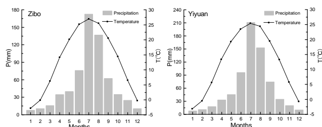
Figure 3. Monthly mean temperature ( T ) and precipitation ( P ) of Zibo (1952–1980) at Zibo Station and Yiyuan (1958–2005) at the Yiyuan Station, two meteorological stations close to the study site (Fig. 1).
