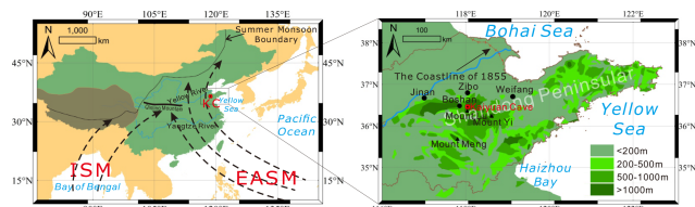
Figure 2. Location of Kaiyuan Cave and Shandong Peninsula in monsoonal China. KC: Kaiyuan Cave ( 36^{\circ}24'32'' [U+2033]N, 118^{\circ}02'05'' [U+2033]E). ISM: India summer monsoon; EASM: East Asia summer monsoon. The dashed black thin line indicates the northwestern boundary of the Asian summer monsoon. The dashed black lines with arrows indicate the routes of the summer monsoon. The dashed black lines with arrows on the left indicate the routes of the summer monsoon. The brown area is the Qinghai–Tibet Plateau. The green and brown area is China, and the yellow area is the other area.
