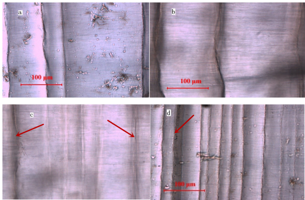
Figure 6. The characteristics of the transmitting laminae in the upper part of stalagmite ky1 show that the thickness of the laminae has obvious variations. The boundary was curved, and the color near the boundary was deeper because of the dark transmitting laminae. The thickness of the laminae shows obvious variations (a), the curve of the boundary of transmitting laminae (b), the color variations of the boundary of transmitting laminae, the arrows indicating the darker boundaries, the boundaries in the middle were obviously whiter (c), dark transmitting laminae (d) (the arrows indicated in the figure).
