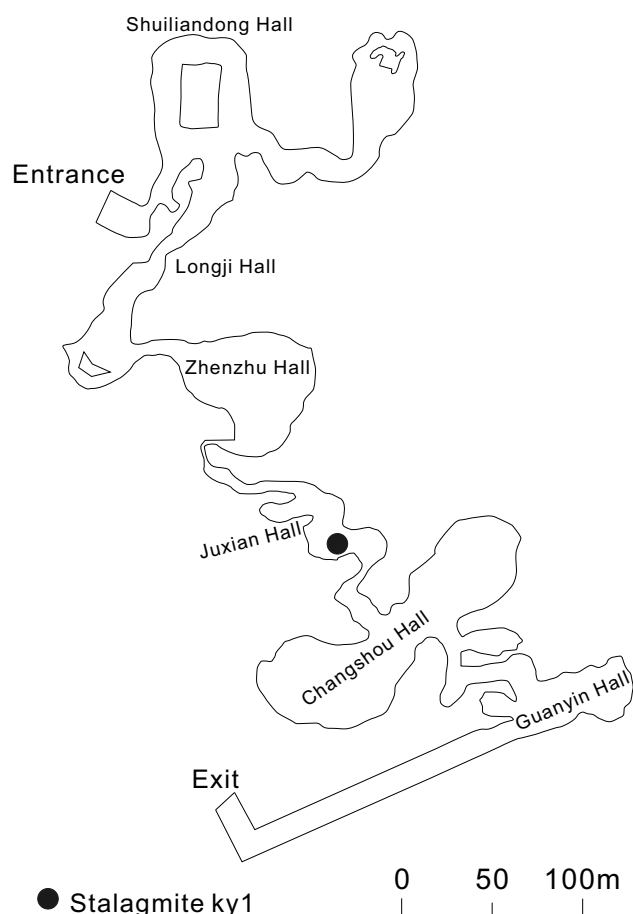
Figure 1. The map of Kaiyuan Cave. The black point is the location where we collected the sample in the cave. The cave has an entrance and an exit and consists of six small halls.
