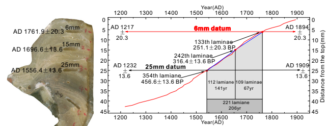
Figure 5. The age model for stalagmite ky1 established by counting of laminae and high-precision dating results with the U- 230 Th technique. This figure is the photo of stalagmite ky1, and the age label was based on high-precision dating results with the U- 230 Th technique on the left. The blue line is the high-precision dating results with the U- 230 Th technique and the connecting lines. The red line is the age scale established by this article. The ages of other laminae were determined by annual laminae counting upward and downward based on the 133rd of the laminae corresponding to the position of 6 mm. The date of which is AD 1762 \pm 20.3 decided by high-precision dating results with the U- 230 Th technique.
