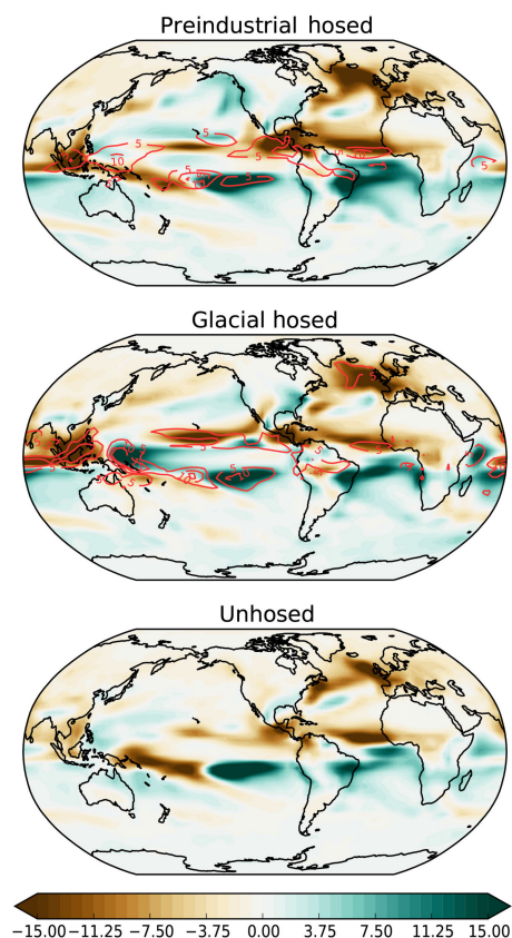
Figure 7. Stadal precipitation anomaly. The top two panels show the precipitation difference between weak and strong AMOC states (as defined in Fig. 3) under preindustrial and glacial boundary conditions, averaged between the four sets of orbital configurations (see Fig. S4 to view all eight hosing simulations individually). Red contours show the standard deviation between the four sets of orbital configurations at 5 \times 10^{-6} \text{ kg m}^{-2} \text{ s}^{-1} intervals. The bottom panel shows the precipitation difference between weak and strong AMOC states (as defined in Fig. 3) in the unhosed simulation. Shading and contours in 10^{-6} \text{ kg m}^{-2} \text{ s}^{-1} .
