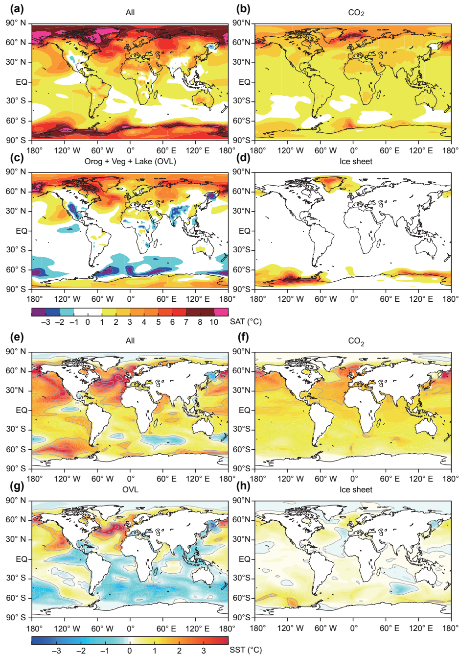
Figure 5. (a) Anomaly in SAT ( ^{\circ}\text{C} ) in Pliocene run relative to pre-industrial run (hereafter All). (b) E400 run minus pre-industrial run ( \text{CO}_2 ), (c) Eo280 run minus pre-industrial run (OVL), and (d) Ei280 run minus pre-industrial run (Ice Sheet), respectively. The anomalies are calculated by averages for the last 50 years of the individual runs. (e–h) Similar to (a–d), but for sea surface temperature (SST; ^{\circ}\text{C} ). Intervals of grey contours are 1.5^{\circ}\text{C} .
