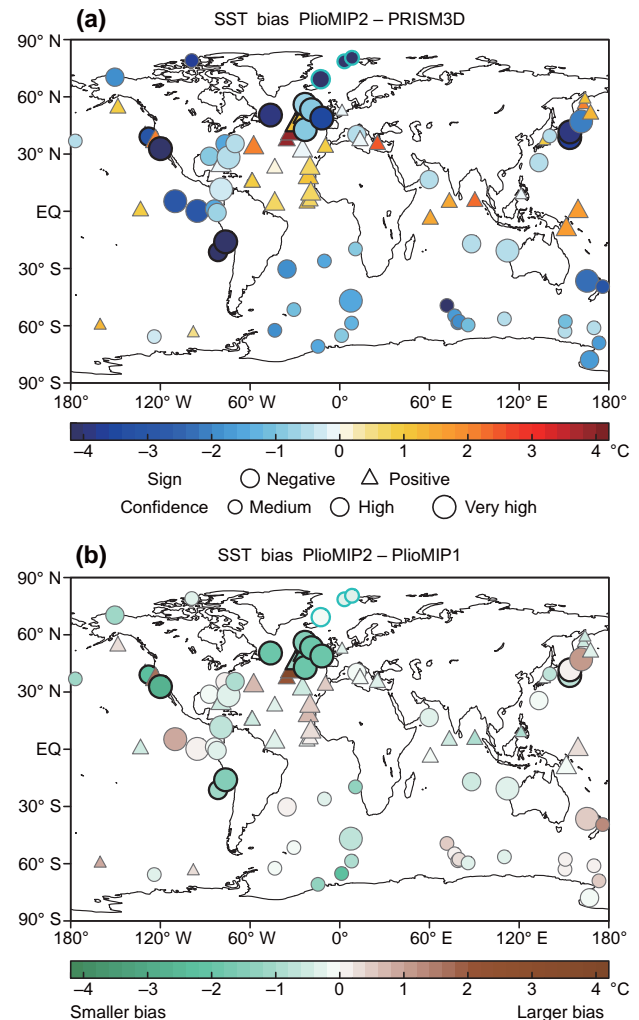
Figure 11. (a) SST bias ( ^{\circ}\text{C} ) in PlioMIP2 Pliocene run compared with PRISM3D proxy-based SST reconstruction (Dowsett et al., 2009). Coloured circles and triangles represent cool and warm biases, respectively. Sizes of plots indicate confidence levels of SST estimate based on chronology, sampling density, sampling quality and performance of quantitative method (Dowsett et al., 2013). Thick black and blue open circles indicate proxy sites in which estimated SST anomalies are large (between 4.0 and 8.9\text{ }^{\circ}\text{C} ) and extremely large ( >8.9\text{ }^{\circ}\text{C} ), respectively. (b) Comparison of SST biases in Pliocene runs between PlioMIP2 and 1. Coloured plots indicate differences in absolute biases between the two.
