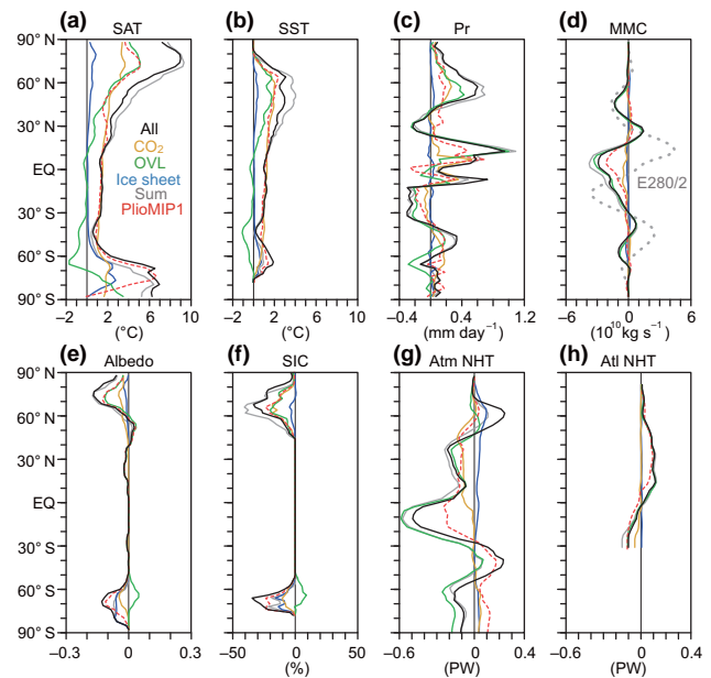
Figure 6. Zonal-mean anomalies in (a) SAT (°C), (b) SST (°C), (c) precipitation (mm day -1 ), (d) mass stream function of mean meridional circulation at 500 hPa level (10 10 kg s -1 ), (e) surface albedo, (f) sea ice concentration (%), (g) northward heat transport due to atmosphere (PW) and (h) the Atlantic (PW). Black, yellow, green, and blue lines represent All, CO 2 , OVL, and Ice Sheet, respectively. Grey line represents Sum. Dashed red lines represent results of AOGCM_NFA run conducted in the identical model in PlioMIP1 (Kamae and Ueda, 2012). Dotted grey line in (d) represents climatology in pre-industrial run multiplied by 0.5.
