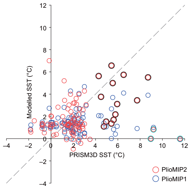
Figure 12. Scatter diagram of proxy-based SST reconstruction ( ^{\circ}\text{C} ) and simulated SST ( ^{\circ}\text{C} ). Red and blue circles represent Pliocene runs in PlioMIP2 and 1, respectively. Thick black and blue open circles are identical to Fig. 11. Dashed grey line represents one-by-one line.
