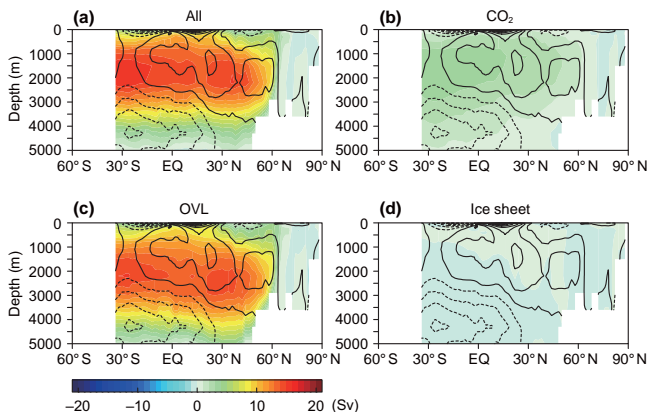
Figure 10. Anomalies in Atlantic meridional overturning circulation (AMOC; shading; Sv). Contours represent climatological overturning circulation in pre-industrial run ( \pm 0, 2, 4, 6, 8 \text{ Sv} ). (a) All, (b) \text{CO}_2 , (c) OVL, and (d) Ice Sheet, respectively.
