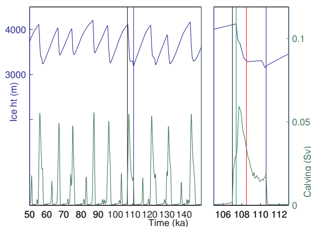
Figure 3. Variability in the ice sheet over Hudson Bay and Hudson Strait. The upper curve shows the average height of the ice sheet over central Hudson Bay (m, blue box in Fig. 2); the lower curve is the flux of ice out of the mouth of Hudson Strait ( 1 \text{ Sv} = 1 \times 10^6 \text{ m}^3 \text{ s}^{-1} ). The left panel shows results for 100 000 years of model run; the right panel zooms in on the event between 105 and 113 kyr.
