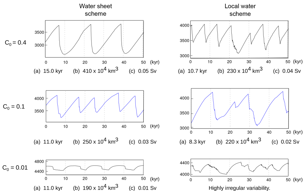
Figure 8. Summary of sensitivity to sliding parameter. We show the height of the ice sheet in the central Hudson Bay for three different values of the sliding parameter and for the two different water schemes. Example statistics for typical events, averaged over the full 100 kyr are also shown; these are (a) the period, (b) the size and (c) the peak calving rate.
