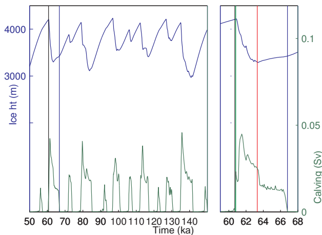
Figure 9. Variability in the ice sheet over Hudson Bay and Hudson Strait using the local water scheme. The upper curve shows the average height of the ice sheet over the central Hudson Bay (m, blue box in Fig. 2); the lower curve is the flux of ice out of the mouth of Hudson Strait ( 1 \text{ Sv} = 1 \times 10^6 \text{ m}^3 \text{ s}^{-1} ). The left panel shows results for 100 000 years of model run; the right panel zooms in on the event between 60 and 68 kyr.
