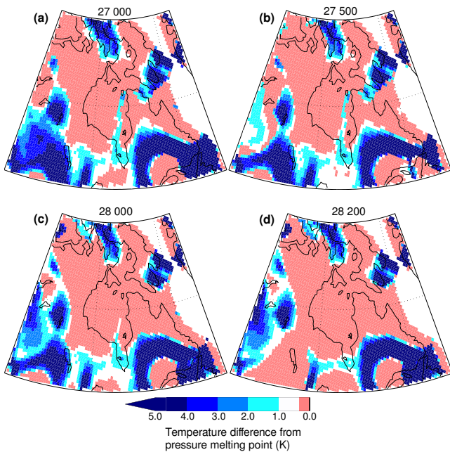
Figure 4. Time slices of the basal temperature field taken at (a) 27 000 years, (b) 27 500 years, (c) 28 000 years and (d) 28 200 years. The times shown are the same as those in Fig. 5. Temperatures are plotted relative to the pressure melting point, with red colours indicating where the ice sheet base is at pressure melting.
