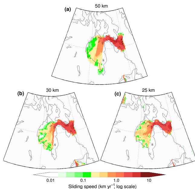
Figure 11. Instantaneous basal sliding speed for model runs at three different resolutions: (a) 50 km, (b) 30 km and (c) 25 km. Colours for speed are plotted on a logarithmic scale.
