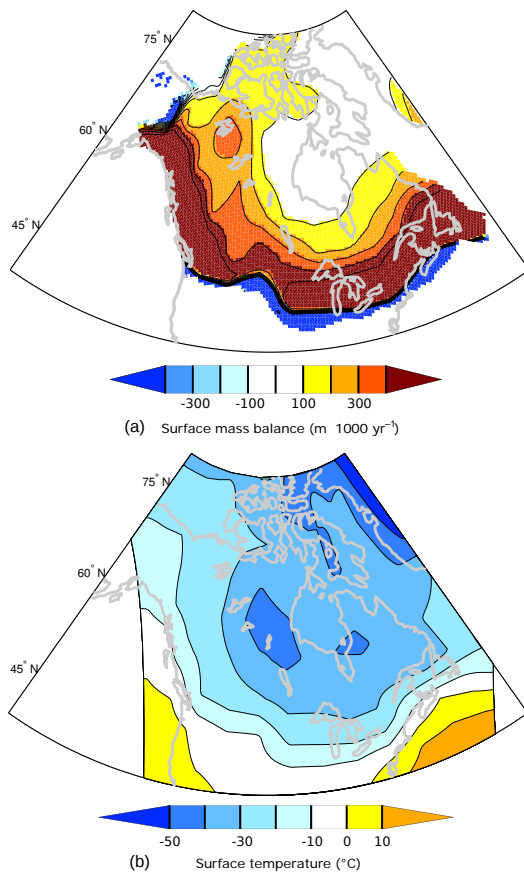
Figure 1. Ice sheet forcing fields. Panel (a) shows the annual average surface mass balance field and panel (b) the annual average surface temperature field.
