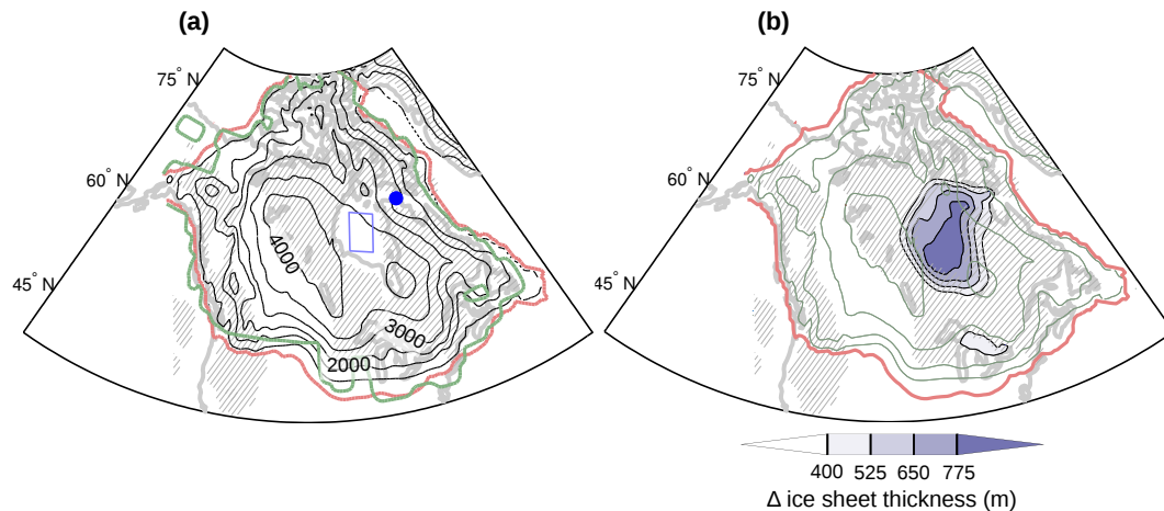
Figure 2. The mean height of the ice sheet (a) and the mean change in topography over a composite Heinrich event (b). In (a) the black contours show the height of the ice sheet; contour interval 500 m. The red contour shows the extent of the ice sheet as modelled by Glimmer; the green contour shows the extent of the ice5g ice sheet (Peltier, 2004). Hatched areas indicate areas of hard bed, where the sliding parameter is very low; the remaining areas are soft bed with higher sliding parameter. The blue square is the region over which the upper curve in Fig. 3 is averaged. The blue dot shows the location from which the time series in Fig. 5 are derived. In (b) we show the composite difference between the ice sheet thickness before and after an HE. The composite is the average over all HEs that occur during the 100 kyr run of the model shown in Fig. 3.
