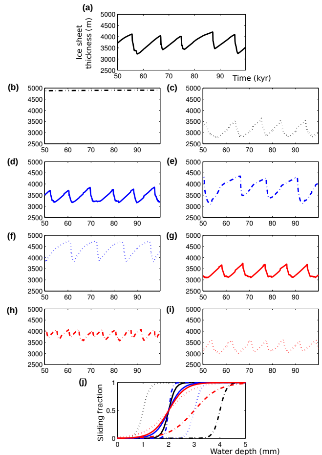
Figure 10. Sensitivity to the parameters (a) and (b) in Eq. (1). The values are presented in Table 2. Panels (a)–(i) show the surface height of the ice sheet averaged over the blue box in Fig. 3. Panel (j) shows the sliding fraction, \frac{C}{C_0} from Eq. (1), as a function of water depth, for the different values. The parameter values in each panel are as follows: (a) a: 2.0 \text{ mm} , b: 0.8 \text{ mm} ; (b) a: 4.0 \text{ mm} , b: 0.8 \text{ mm} ; (c) a: 1.0 \text{ mm} , b: 0.8 \text{ mm} ; (d) a: 2.0 \text{ mm} , b: 1.6 \text{ mm} ; (e) a: 2.0 \text{ mm} , b: 0.4 \text{ mm} ; (f) a: 3.0 \text{ mm} , b: 0.8 \text{ mm} ; (g) a: 2.0 \text{ mm} , b: 2.0 \text{ mm} ; (h) a: 3.0 \text{ mm} , b: 3.0 \text{ mm} ; (i) a: 2.0 \text{ mm} , b: 3.0 \text{ mm} .
