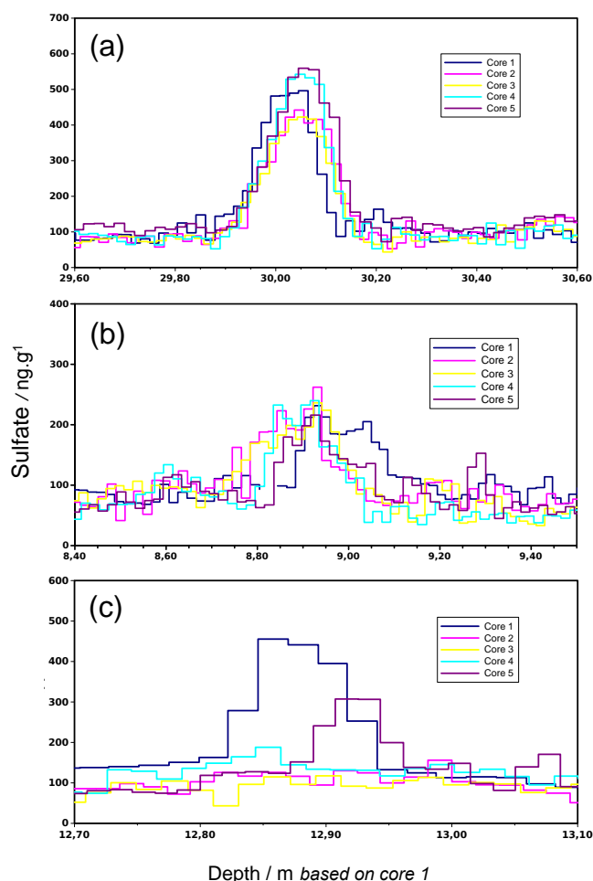
Figure 3. Kuwaie (a), Krakatua (b) and Tambora (c) sulfate concentration profiles after depth synchronization. All peaks are within a 20 cm uncertainty, enabling us to clearly attribute each occurrence to a single event.
