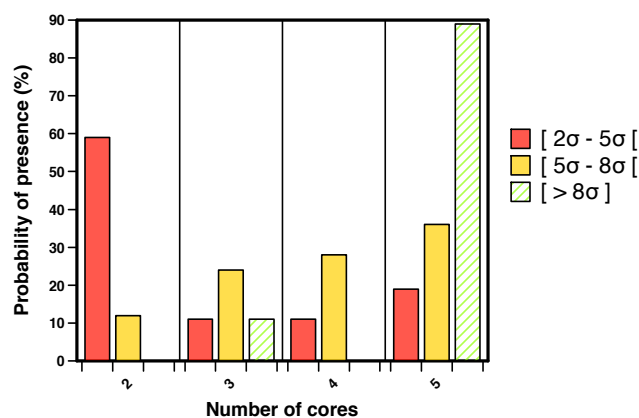
Figure 7. Peaks probability to be detected in two, three, four or five cores, as a function of their flux. The three categories of fluxes are defined by peak flux value, relatively to the average background flux, and quantified by x time (2, 5 and 8) the flux standard deviation (calculated for a 30 ppb standard deviation in concentrations). At flux above background flux + 8\sigma , there is a 90 % chance of detecting the volcanic peak in each core of a population of five cores. On the other hand, at flux below background flux + 5\sigma , there is a 60 % probability of the volcanic peak being detected in two cores only among the five-core population. This highlights that replicate cores are particularly useful to avoid missing small to intermediate peaks in a record.
