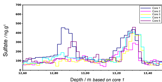
Figure 8. Close look at UE 1809 and Tambora (1815) events showing the absence of the Tambora event in two out of the five cores. This figure illustrates the possibility of missing major volcanic eruptions when a single core is used.
