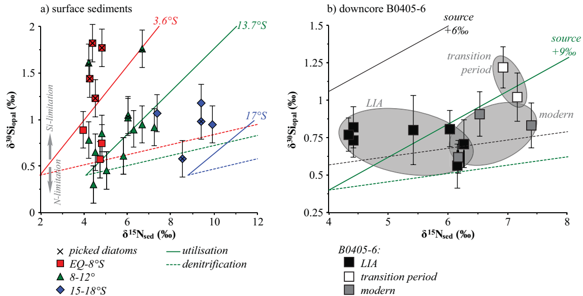
Figure 4. Relationship between \delta^{15}\text{N}_{\text{sed}} versus \delta^{30}\text{Si}_{\text{opal}} for (a) surface sediments and (b) downcore data from core B0405-6. The crosses in (a) indicate \delta^{30}\text{Si} data obtained from hand-picked diatoms, which reflect a different growth season than bulk \delta^{30}\text{Si}_{\text{opal}} and which are influenced by stronger \text{Si}(\text{OH})_4 limitation (higher \delta^{30}\text{Si} ) (Ehlert et al., 2012). The solid lines reflect theoretical utilisation (assuming 1 : 1 utilisation of \text{Si}(\text{OH})_4 and \text{NO}_3^- by the diatoms) and the dashed lines mark the theoretically expected line for denitrification, which represent the expected signal preserved in the sediments, based on present-day measurements: \delta^{30}\text{Si} source signature and enrichment factor \varepsilon_{\text{diatom}-\text{Si}(\text{OH})_4} are always +1.5 ‰ (Ehlert et al., 2012) and -1.1 ‰ (De La Rocha et al., 1997), respectively. \delta^{15}\text{N}_{\text{sed}} source signature and \varepsilon_{\text{organic}-\text{NO}_3^-} vary with latitude (Mollier-Vogel et al., 2012); in the north at 3.6° S, source signature and \varepsilon are +5.7 and -3.7 ‰ (red curves); along the central shelf at 13.7° S, source signature and \varepsilon are +8.9 and -4.8 ‰ (green curves); and in the south at 17° S, source signature and \varepsilon were measured to be +14.5 and -5.7 ‰ (blue curves), respectively. The samples are colour-coded according to their location on the shelf and relative to the \text{NO}_3^- utilisation/ \text{NO}_3^- loss that they experienced. Data points that plot above the utilisation curves reflect predominant \text{Si}(\text{OH})_4 limitation, whereas data points below record stronger \text{NO}_3^- limitation. The isotopic enrichment during denitrification was always set to be +20 ‰. For the downcore data (b) two different assumed source signatures are displayed: +9 ‰ (green lines, corresponding to the modern conditions along the central shelf region in a) and +6 ‰ (grey lines). Data points are colour-coded according to the respective time periods (black: LIA; white: transition period; grey: modern). Error bars represent 2\sigma_{(\text{sd})} external reproducibilities.
