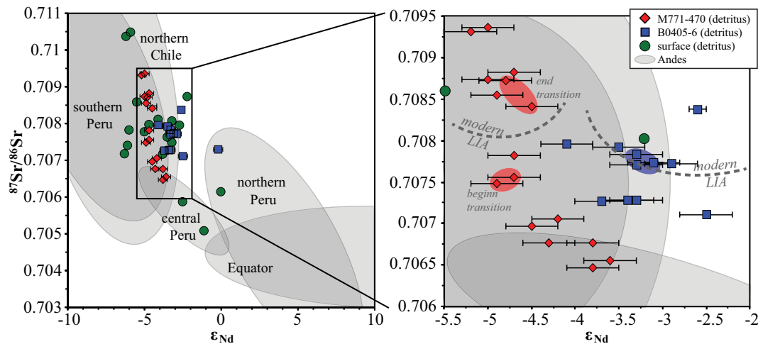
Figure 6. \epsilon_{\text{Nd}} detritus versus ^{87}\text{Sr}/^{86}\text{Sr} detritus for core M771-470 (red diamonds) and B0405-6 (blue squares). Error bars represent 2\sigma_{(\text{sd})} external reproducibilities. The green dots are data obtained from surface sediment samples at different sites on the Peruvian shelf. The grey shadings indicate potential sources and provenance end members of the detrital material.
