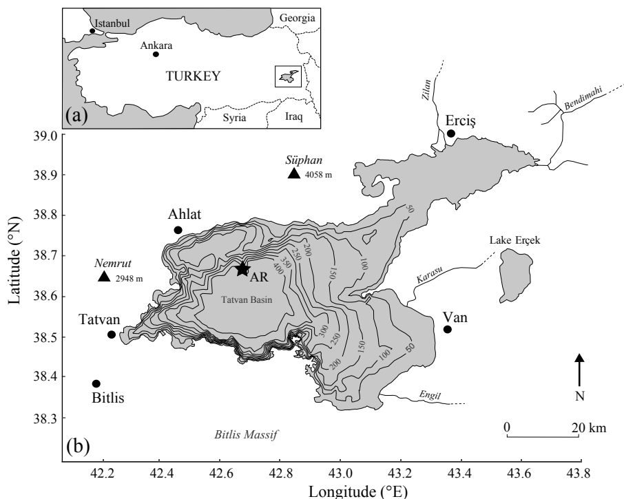
Figure 1. (a) Location of Lake Van in eastern Anatolia (Turkey) and (b) the bathymetry of Lake Van including the main ICDP drill site Ahlat Ridge (AR, black star). Major cities (black dots) and rivers are represented. The black triangle indicates the positions of the active volcanoes Nemrut and Süphan. The Bitlis Massif in the south reaches up to 3500 m a.s.l.
