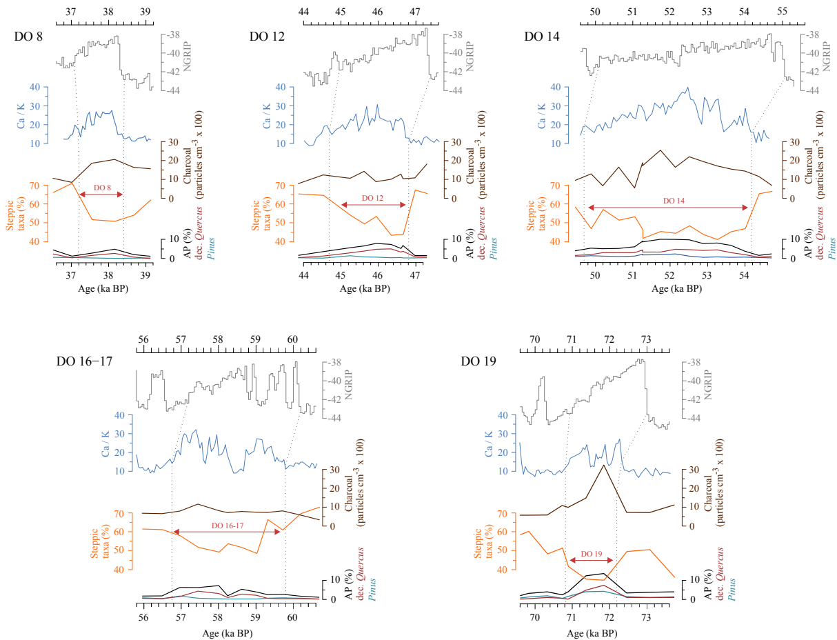
Figure 5. The most pronounced Dansgaard–Oeschger events DO 8, DO 12, DO 14, DO 16–17 and DO 19 are plotted in extra graphs, demonstrating a good correlation between the vegetation and environmental dynamics in eastern Anatolia and the \delta^{18}\text{O} -profile from the Greenland ice core sequence (NGRIP members, 2004); Ca / K ratio after Kwiciczen et al. (2014); microscopic charcoal concentration (particles \text{cm}^{-3} , this study); selected Lake Van arboreal pollen (AP, Pinus , deciduous Quercus in %, this study). The term “Steppic taxa” includes only major dry-adapted plants such as Chenopodiaceae and Artemisia .
