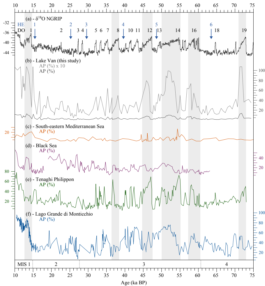
Figure 4. Regional comparison of vegetation dynamics and climate variability in the central and eastern Mediterranean area and Black Sea region concerning Dansgaard–Oeschger cycles (DO) and Heinrich events (HE). The gray bars represent the most pronounced DO interstadials DO 19, 17–16, 14, 12, 8, and DO 1, which are discussed in Sect. 5.2. (a) \delta^{18}\text{O} -profile from NGRIP ice core, Greenland (NGRIP members, 2004), labeled with DO 1 to 19 and HE 1 to HE 6 (Bond et al., 1993); (b) Lake Van arboreal pollen record (AP in %, black line) with 10-fold exaggeration (gray line); (c) marine arboreal pollen record (Core 9509) obtained from the south-eastern Levantine Basin (south-eastern Mediterranean Sea; Langgut et al., 2011); (d) AP record from the SE Black Sea (core 22-GC3 for the period from 10 to 18 ka BP after Shumilovskikh et al. (2012) and core 25-GC1 for the sequence between 19 and 63 ka BP (Shumilovskikh et al., 2014); (e) arboreal pollen record from Tenaghi Philippon, Greece (Müller et al., 2011); (f) AP record from Lago Grande di Monticchio, southern Italy (Allen et al., 1999). MIS – Marine Isotope Stage.
