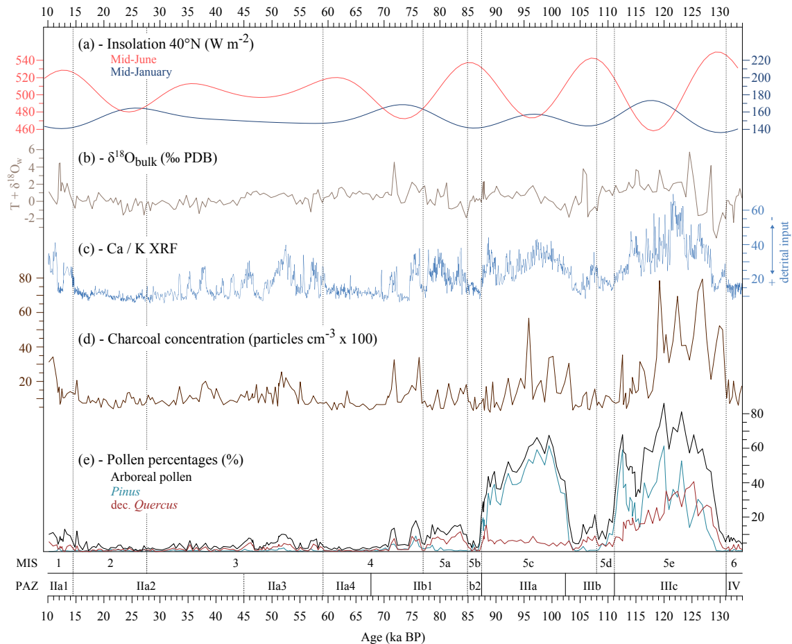
Figure 3. Comparative study of the Lake Van paleoenvironmental sequence encompassing the last glacial–interglacial cycle. (a) Mid-June and Mid-January insolation at 40^{\circ} N ( \text{W m}^{-2} ; Berger, 1978; Berger et al., 2007); (b) Lake Van oxygen isotope record ( \delta^{18}\text{O}_{\text{bulk}} in ‰ PDB) of autochthonous precipitated carbonates. Shown is the temperature ( T ) and the isotopic composition ( \delta^{18}\text{O}_{\text{w}} ) of the epilimnion; (c) calcium/potassium ratio ( \text{Ca} / \text{K} ) after Kwiecien et al. (2014); (d) microscopic charcoal concentration ( \text{particles cm}^{-3} ) from 10–110 ka BP (this study) and from 110–135 ka BP (MIS 5e; Pickarski et al. 2015); (e) selected Lake Van arboreal pollen percentages (AP, Pinus , deciduous Quercus ) from 10 and 110 ka BP (this study) and from 110–135 ka BP described in Pickarski et al. (2015). MIS – Marine Isotope Stage; PAZ – Pollen assemblage zone.
