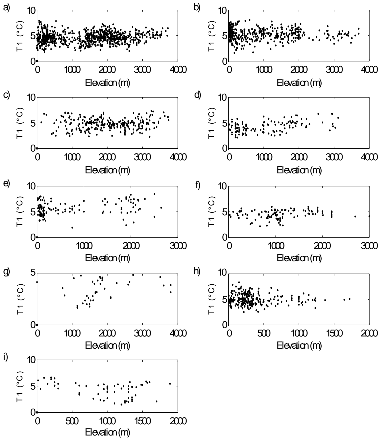
Fig. S2. Comparison of the site values of the threshold temperature T_1 at corresponding elevations for different tree genera: a) pine, b) spruce, c) fir, d) hemlock, e) larch, f) cedar, g) juniper, h) oak, and i) nothofagus.
