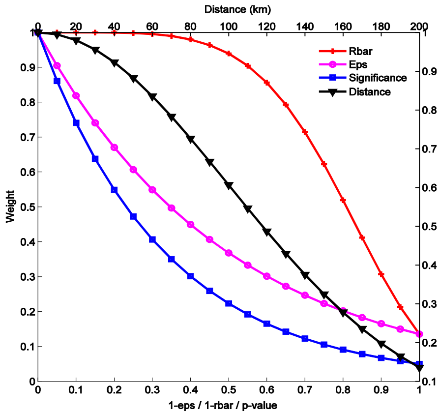
Fig. S1. Weight functions for tree-ring chronologies located within a 200 km search circle around
