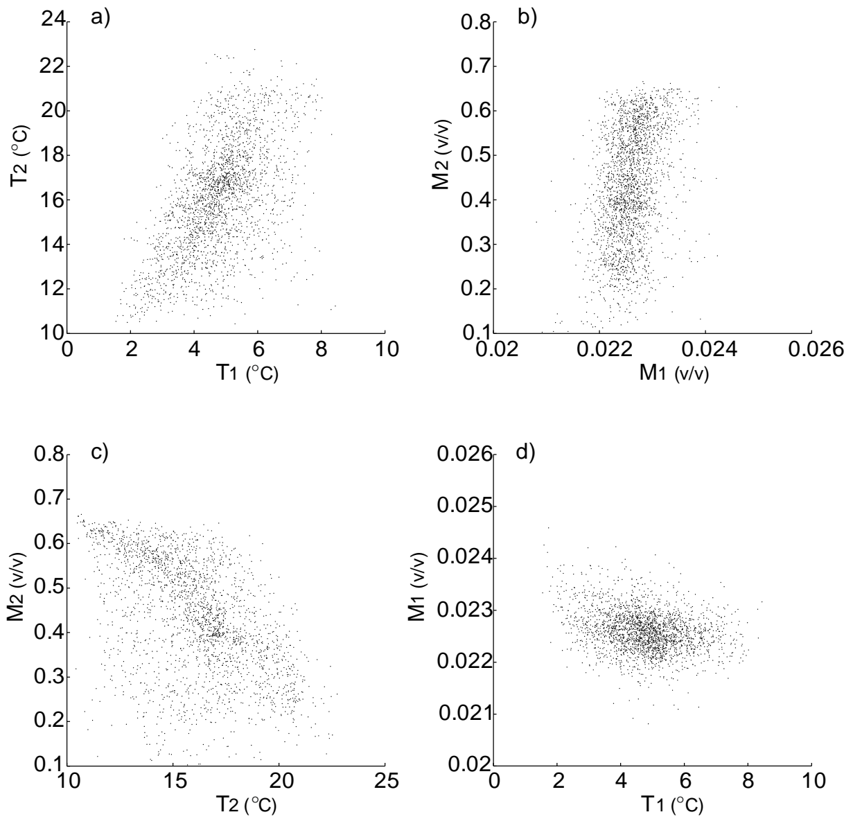
Fig. S3. Scatterplots of joint posterior relationships at each site between parameters a) T_1 and T_2 , b) M_1 and M_2 , c) T_2 and M_2 , and d) T_1 and M_1 .
